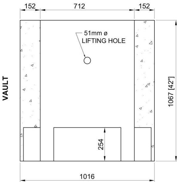
SECTION VIEW
