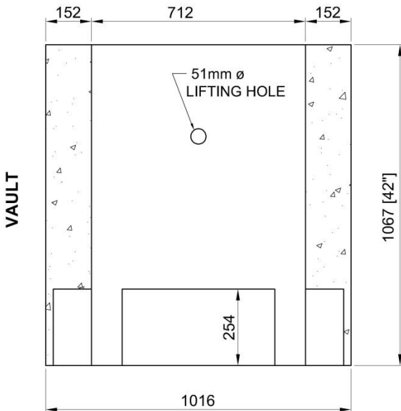
SECTION VIEW
